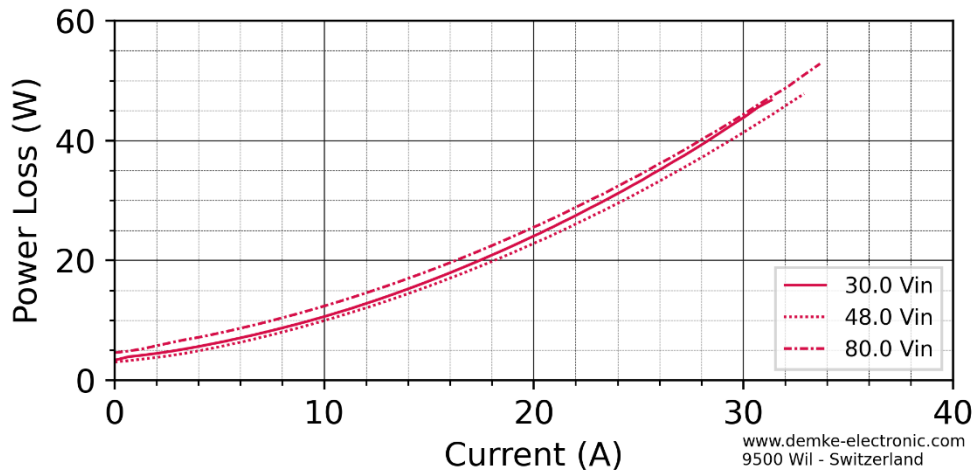
Figure 4: Power Loss over current of the DC-Transformer 767UH-13.8-SD
