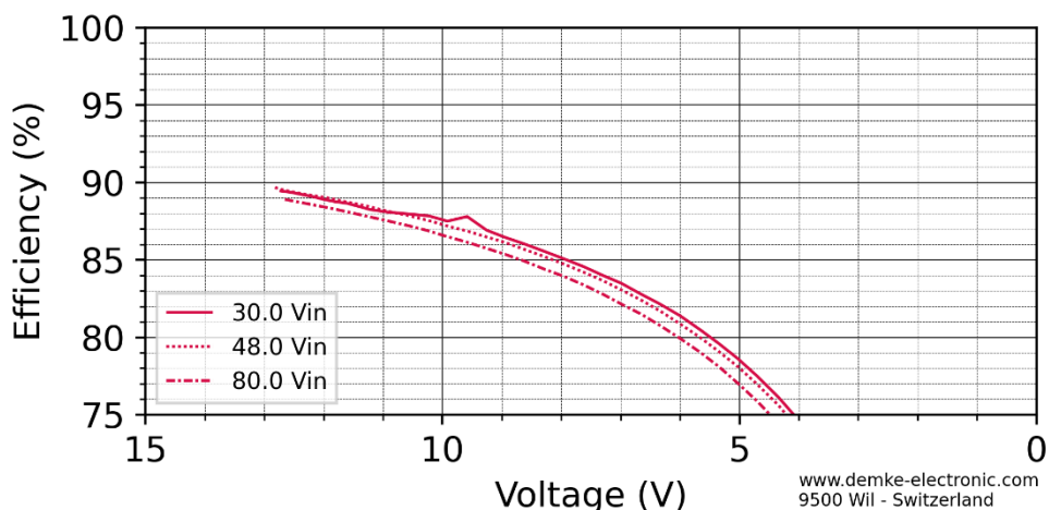
Figure 3 Efficiency in the constant current range of the DC-Transformer 767UH-13.8-SD
