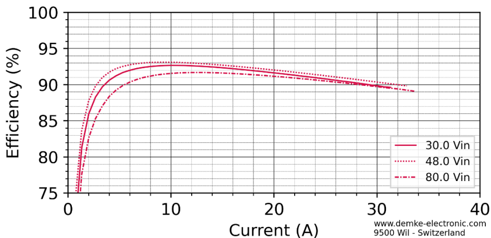
Figure 2 Efficiency in the constant voltage range of the DC-Transformer 767UH-13.8-SD
