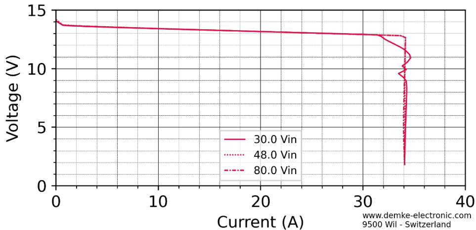
Figure 1 Voltage against current of the DC-Transformer 767UH-13.8-SD
