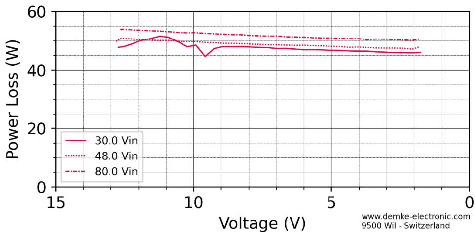
Figure 5: Power Loss over voltage of the DC-Transformer 767UH-13.8-SD
