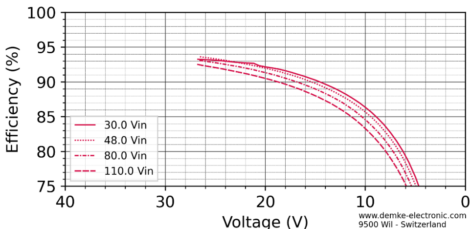
Figure 3 Efficiency in the constant current range of the DC-Transformer 767UH-27.6-SD
