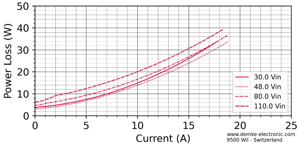
Figure 4: Power Loss over current of the DC-Transformer 767UH-27.6-SD
