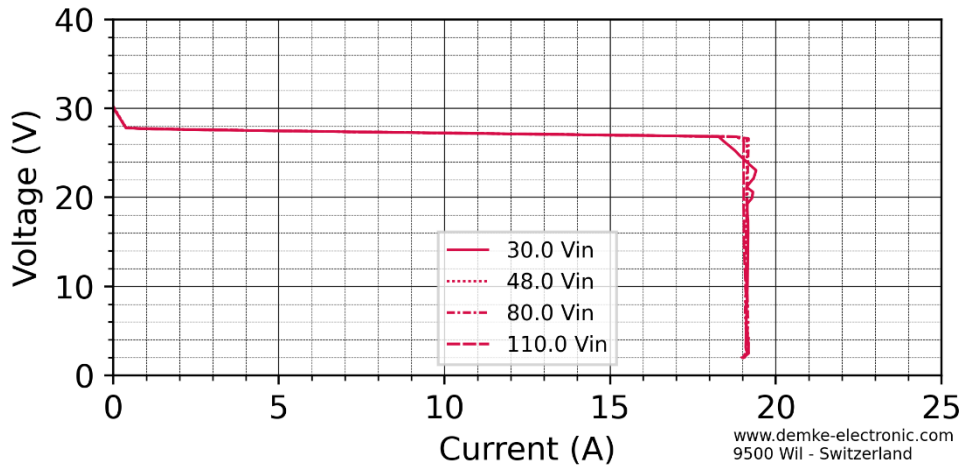
Figure 1 Voltage against current of the DC-Transformer 767UH-27.6-SD
