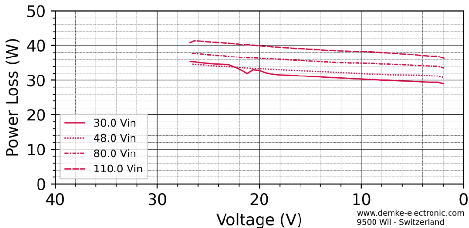
Figure 5: Power Loss over voltage of the DC-Transformer 767UH-27.6-SD
