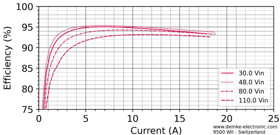
Figure 2 Efficiency in the constant voltage range of the DC-Transformer 767UH-27.6-SD
