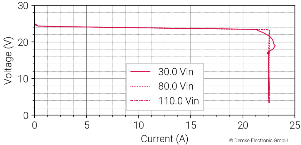
Figure 1 Voltage against current of the DC-Transformer 767UH-24-SD
