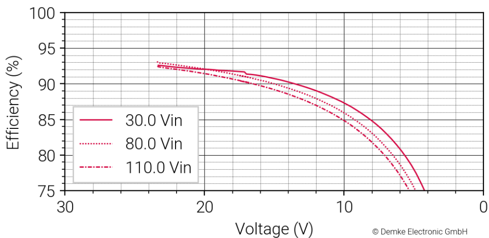
Figure 3 Efficiency in the constant current range of the DC-Transformer 767UH-24-SD
