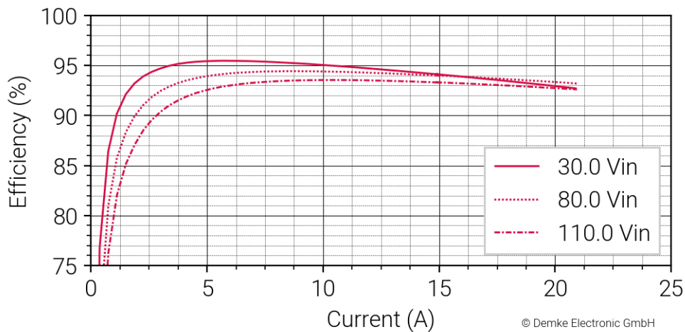
Figure 2 Efficiency in the constant voltage range of the DC-Transformer 767UH-24-SD
