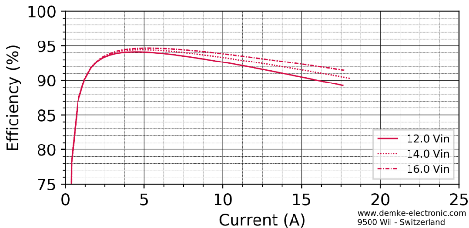
Figure 2 Efficiency in the constant voltage range of the DC-Transformer 729-24-SD
