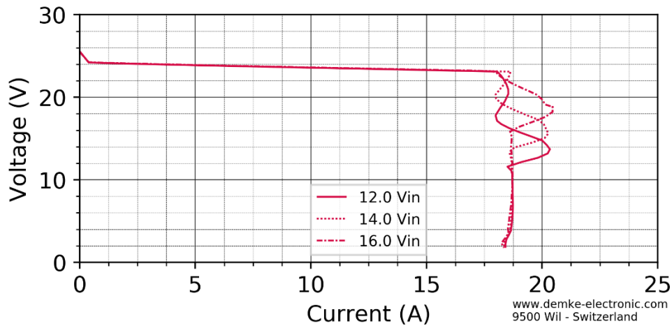
Figure 1 Voltage against current of the DC-Transformer 729-24-SD
