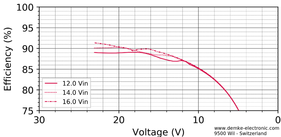
Figure 3 Efficiency in the constant current range of the DC-Transformer 729-24-SD
