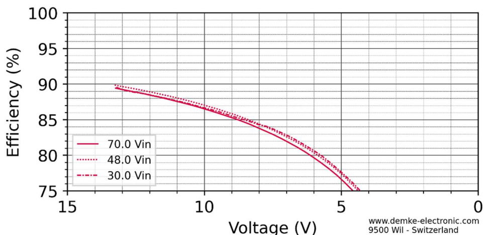
Figure 3 Efficiency in the constant current range of the DC-Transformer 367-13.8-SD
