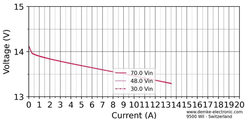
Figure 6: Voltage in CV-mode of the DC-Transformer 367-13.8-SD
