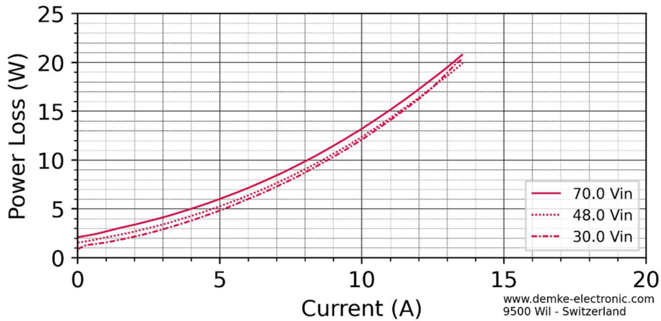
Figure 4: Power Loss over current of the DC-Transformer 367-13.8-SD
