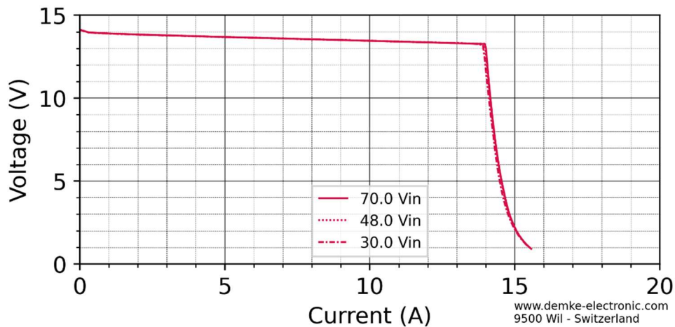
Figure 1 Voltage against current of the DC-Transformer 367-13.8-SD
