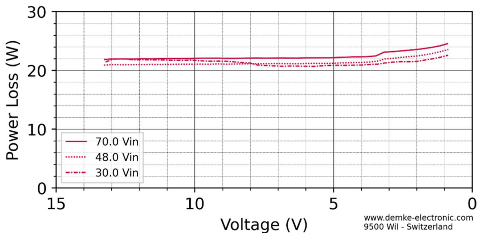
Figure 5: Power Loss over voltage of the DC-Transformer 367-13.8-SD
