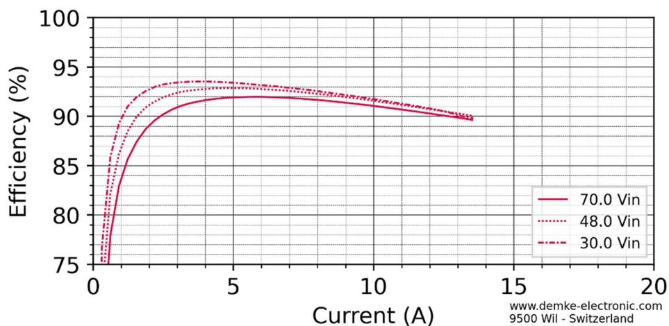
Figure 2 Efficiency in the constant voltage range of the DC-Transformer 367-13.8-SD
