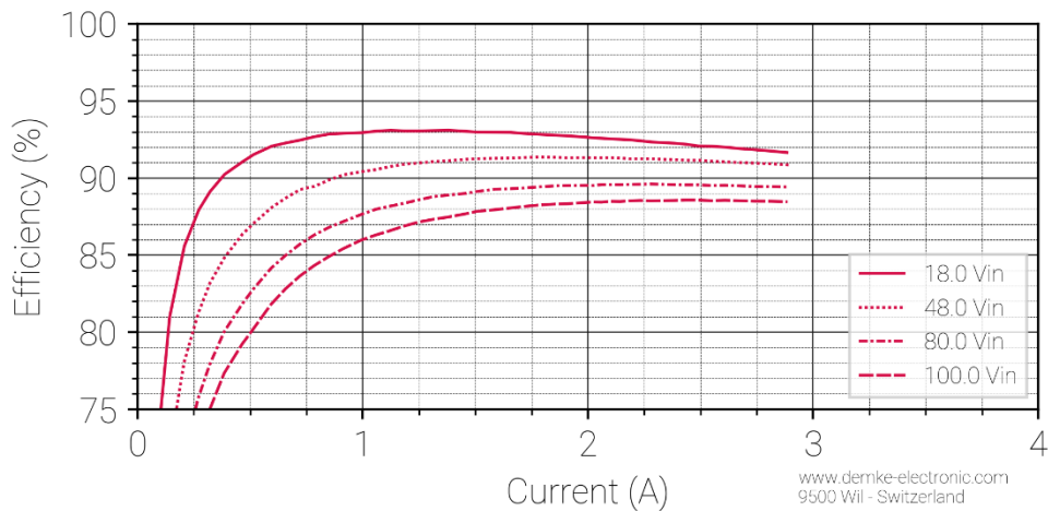
Figure 2 Efficiency in the constant voltage range of the DC-Transformer 334W-19-SD
