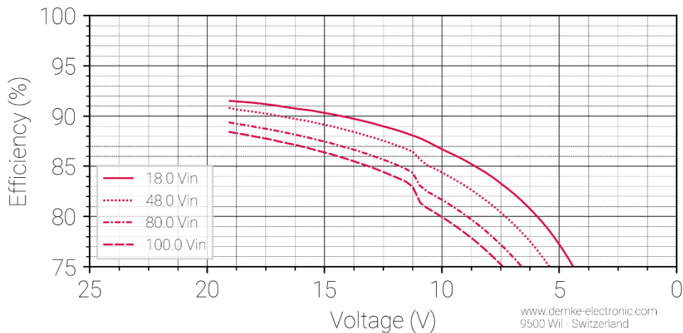
Figure 3 Efficiency in the constant current range of the DC-Transformer 334W-19-SD
