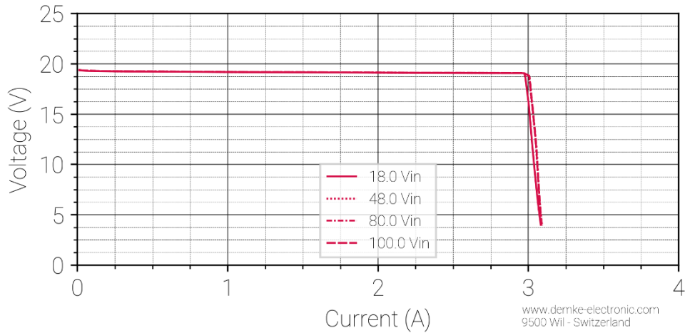
Figure 1 Voltage against current of the DC-Transformer 334W-19-SD
