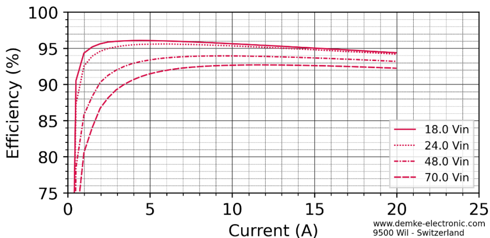
Figure 2 Efficiency in the constant voltage range of the DC-Transformer 162E-13.8-SD
