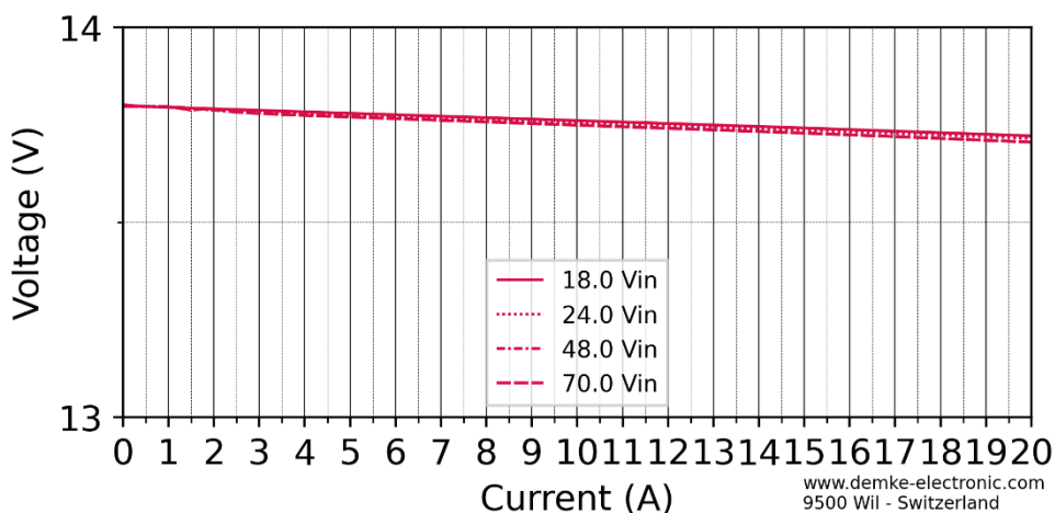
Figure 6: Voltage in CV-mode of the DC-Transformer 162E-13.8-SD
