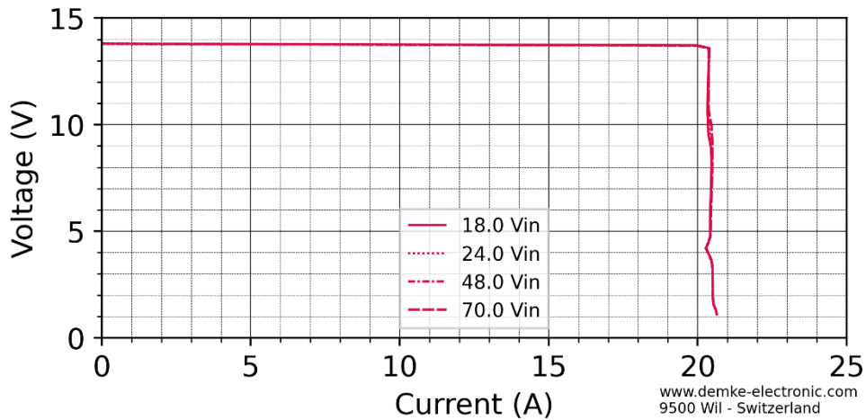
Figure 1 Voltage against current of the DC-Transformer 162E-13.8-SD
