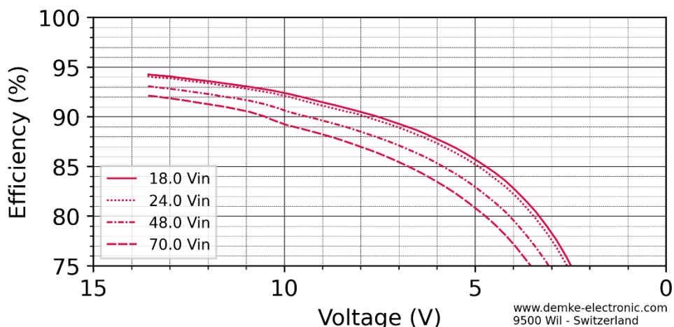
Figure 3 Efficiency in the constant current range of the DC-Transformer 162E-13.8-SD
