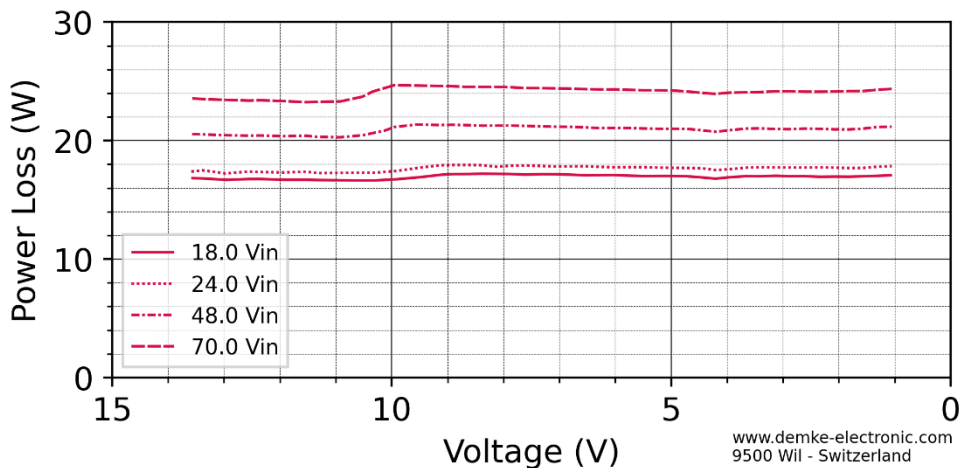
Figure 5: Power Loss over voltage of the DC-Transformer 162E-13.8-SD
