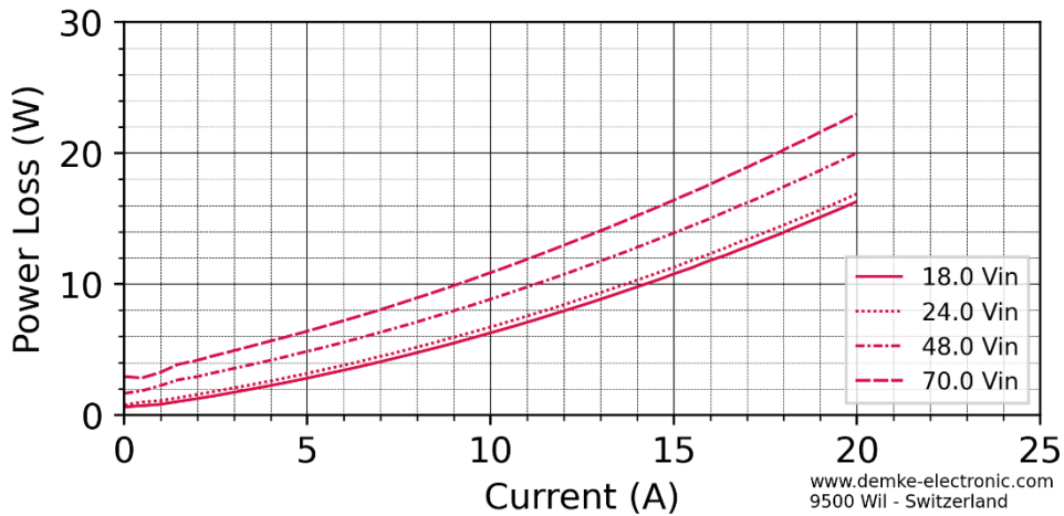
Figure 4: Power Loss over current of the DC-Transformer 162E-13.8-SD
