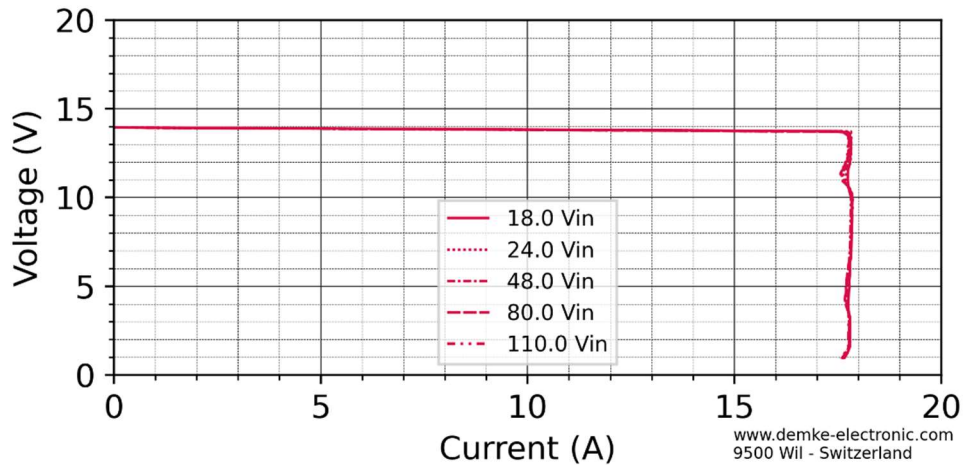
Figure 1 Voltage against current of the DC-Transformer 154DH-13.8-0N
