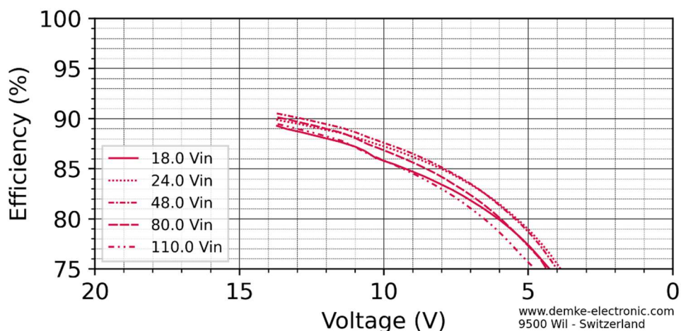
Figure 3 Efficiency in the constant current range of the DC-Transformer 154DH-13.8-0N
