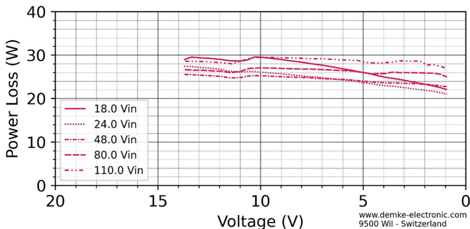
Figure 5: Power Loss over voltage of the DC-Transformer 154DH-13.8-ON
