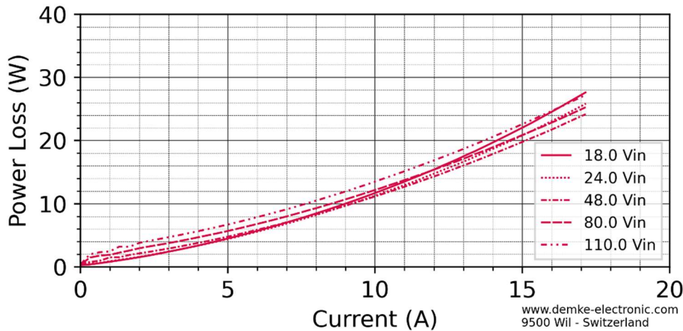
Figure 4: Power Loss over current of the DC-Transformer 154DH-13.8-ON
