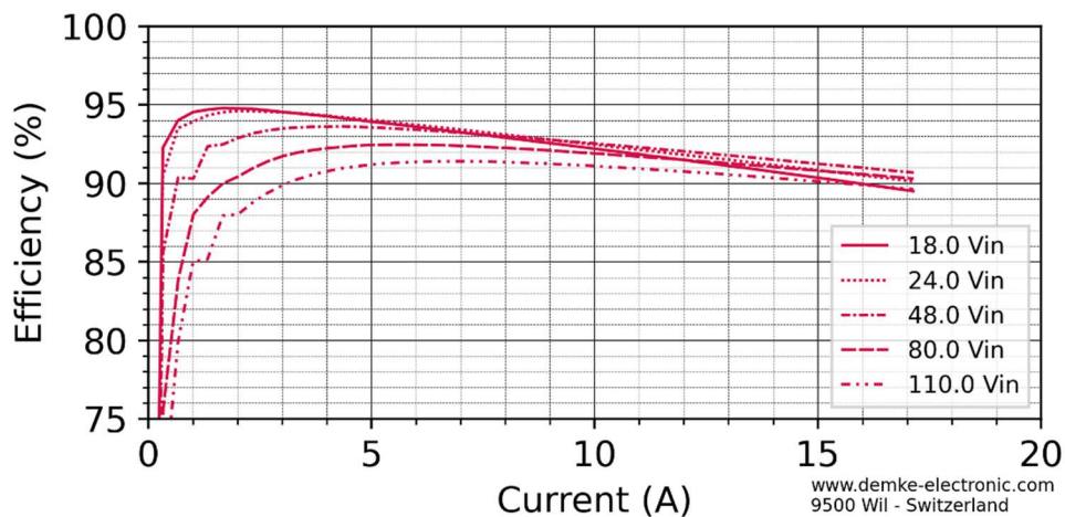
Figure 2 Efficiency in the constant voltage range of the DC-Transformer 154DH-13.8-0N
