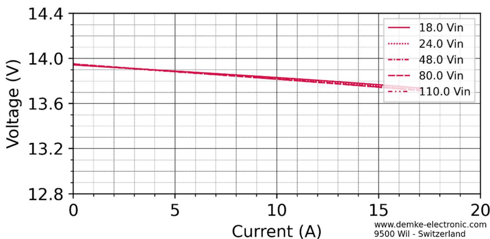
Figure 6: Voltage in CV-mode of the DC-Transformer 154DH-13.8-ON
