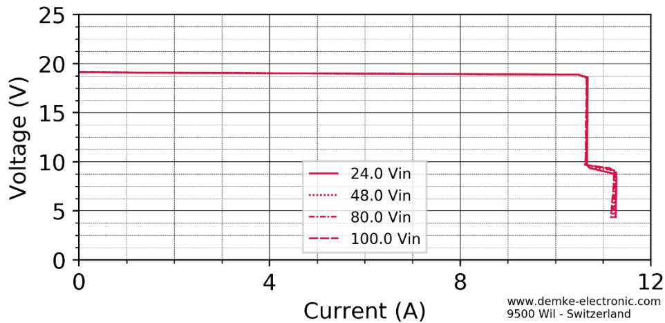
Figure 1 Voltage against current of the DC-Transformer 145-19-SD
