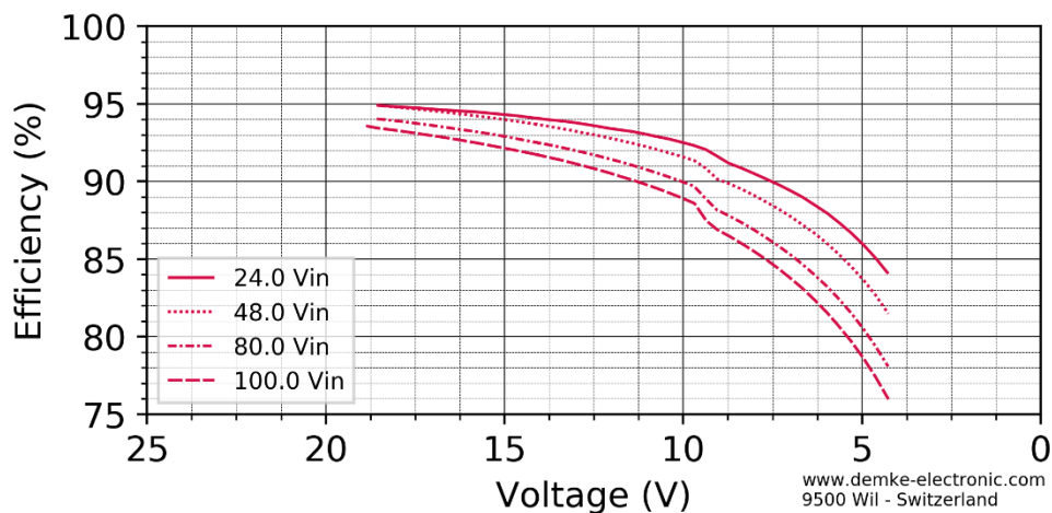
Figure 3 Efficiency in the constant current range of the DC-Transformer 145-19-SD
