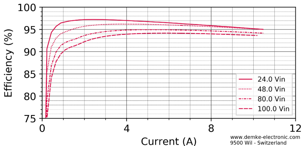
Figure 2 Efficiency in the constant voltage range of the DC-Transformer 145-19-SD
